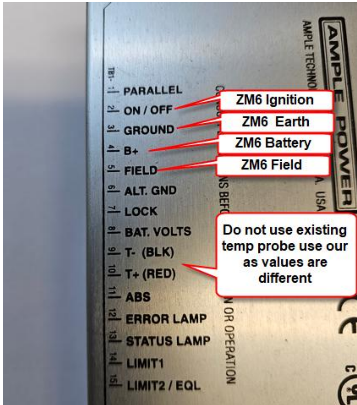
SARV3-12P swap over to ZM6 P switching version
