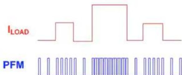
Graph showing pulse frequency modulation versus load
